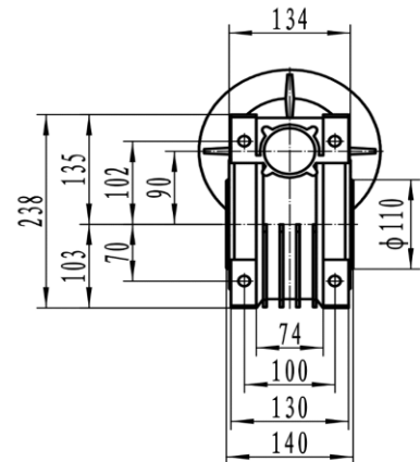
Output shaft hole
